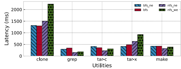
Fig. 10: Task latency of various Linux utilities, with client caching (top) and without (bottom).
