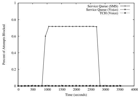
Fig. 11. Blocking for a sector implementing WFQ. Voice calls are unaffected by the attack, whereas the majority of text messages are dropped.
