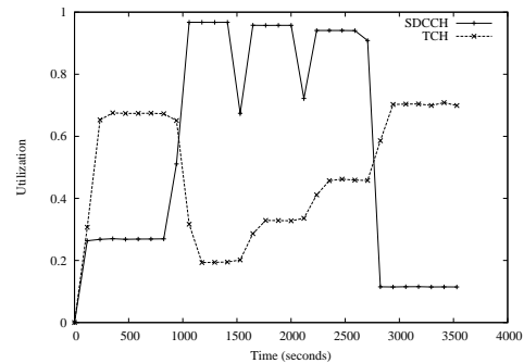
Fig. 18. Channel utilization under DRP
