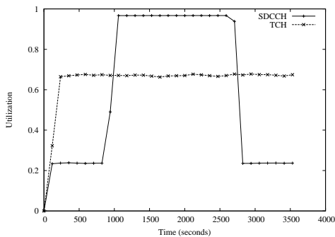
Fig. 20. Channel utilization under DCA
