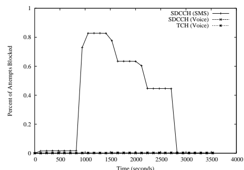
Fig. 22. Blocking for a sector combining DRP and SRP.
