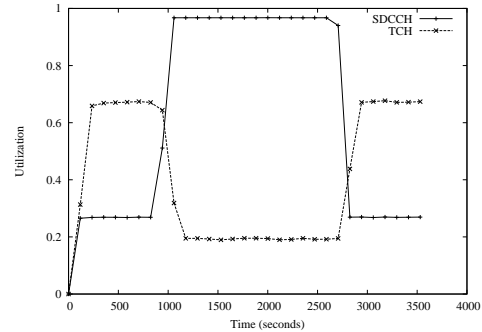
Fig. 8. The utilization of SDCCHs and TCHs for an attack exhibiting a Poisson interarrival at a rate of 495 messages/second.
