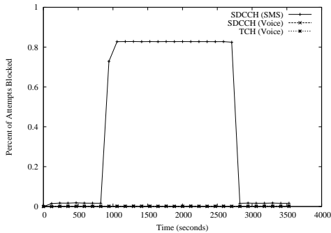
Fig. 15. Blocking for a sector implementing SRP
