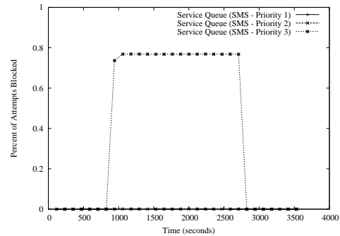
Fig. 13. Blocking for a sector implementing WRED. Unlike WFQ, only Internet-originated text messages are dropped.
