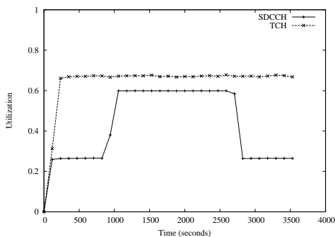
Fig. 16. Channel utilization under SRP
