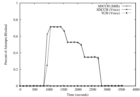
Fig. 17. Blocking for a sector implementing DRP
