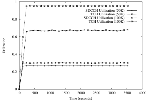
Fig. 4. Channel utilization in a network with a variety of traffic intensities.
