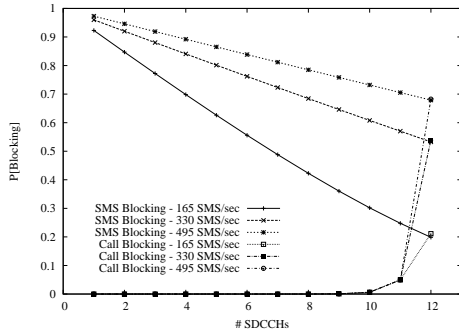
Fig. 9. Blocking probabilities for a system implementing SRP. We vary the number of SDCCHs that will accept SMS requests from 1 to 12(all).
