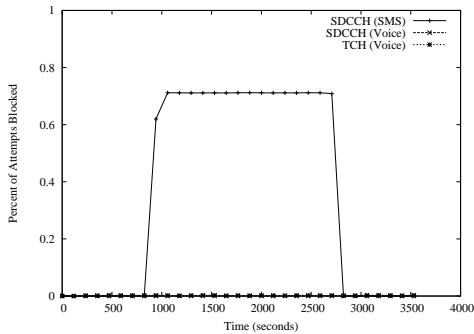
Fig. 19. Blocking for a sector implementing DCA
